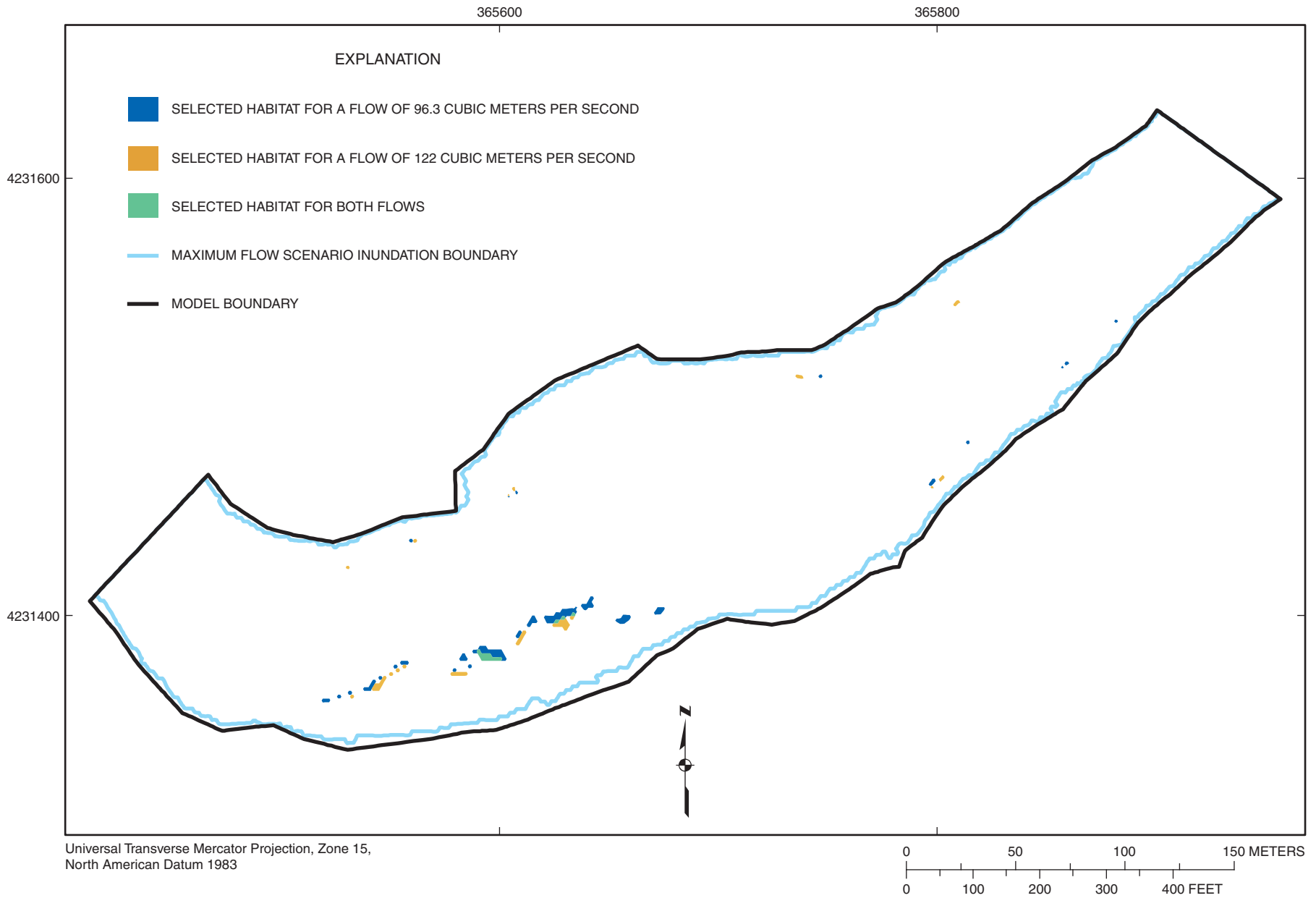
Figure 4-11. Selected habitat area distribution for habitat category 1 (suckermouth minnow) at flows of 96.3 and 122 cubic meters per second at Marais des Cygnes River site MDC2.
